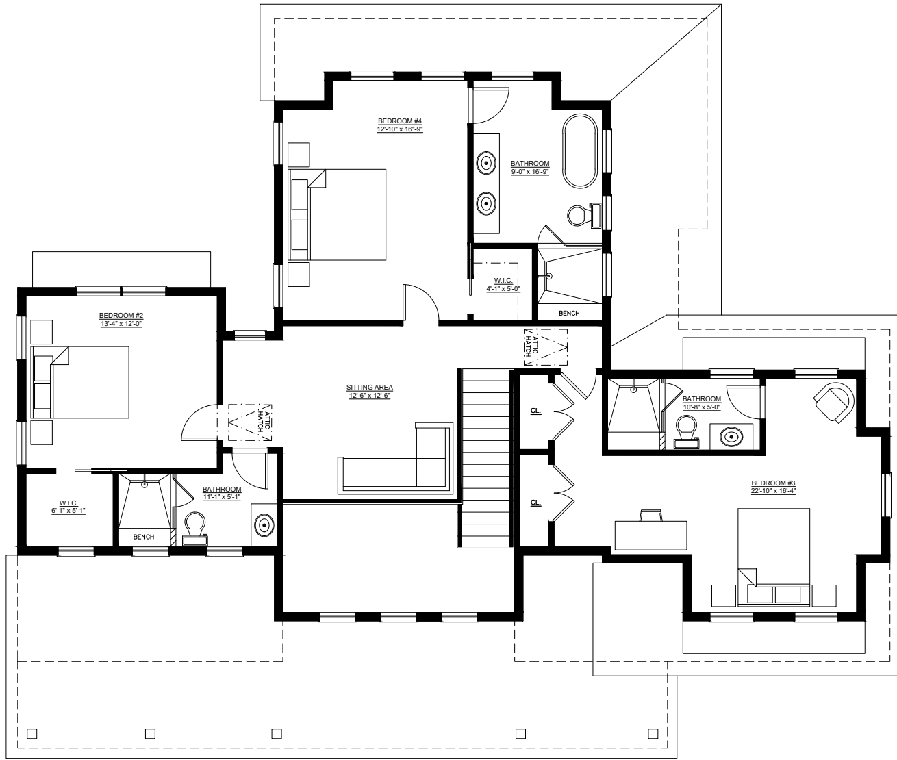
2045 WILLOW SECOND FLOOR
