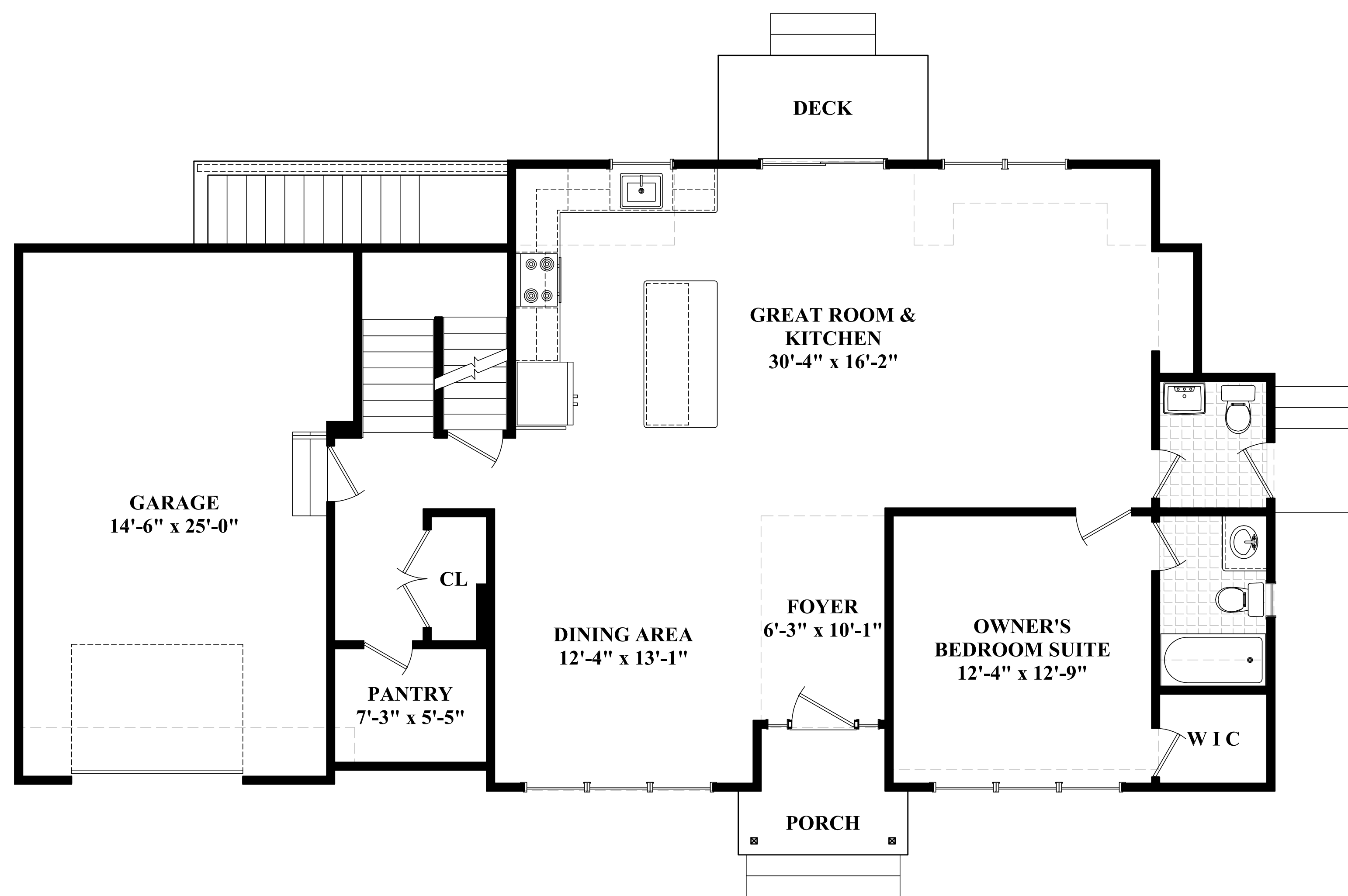
THE CATHERINE FIRST STORY
