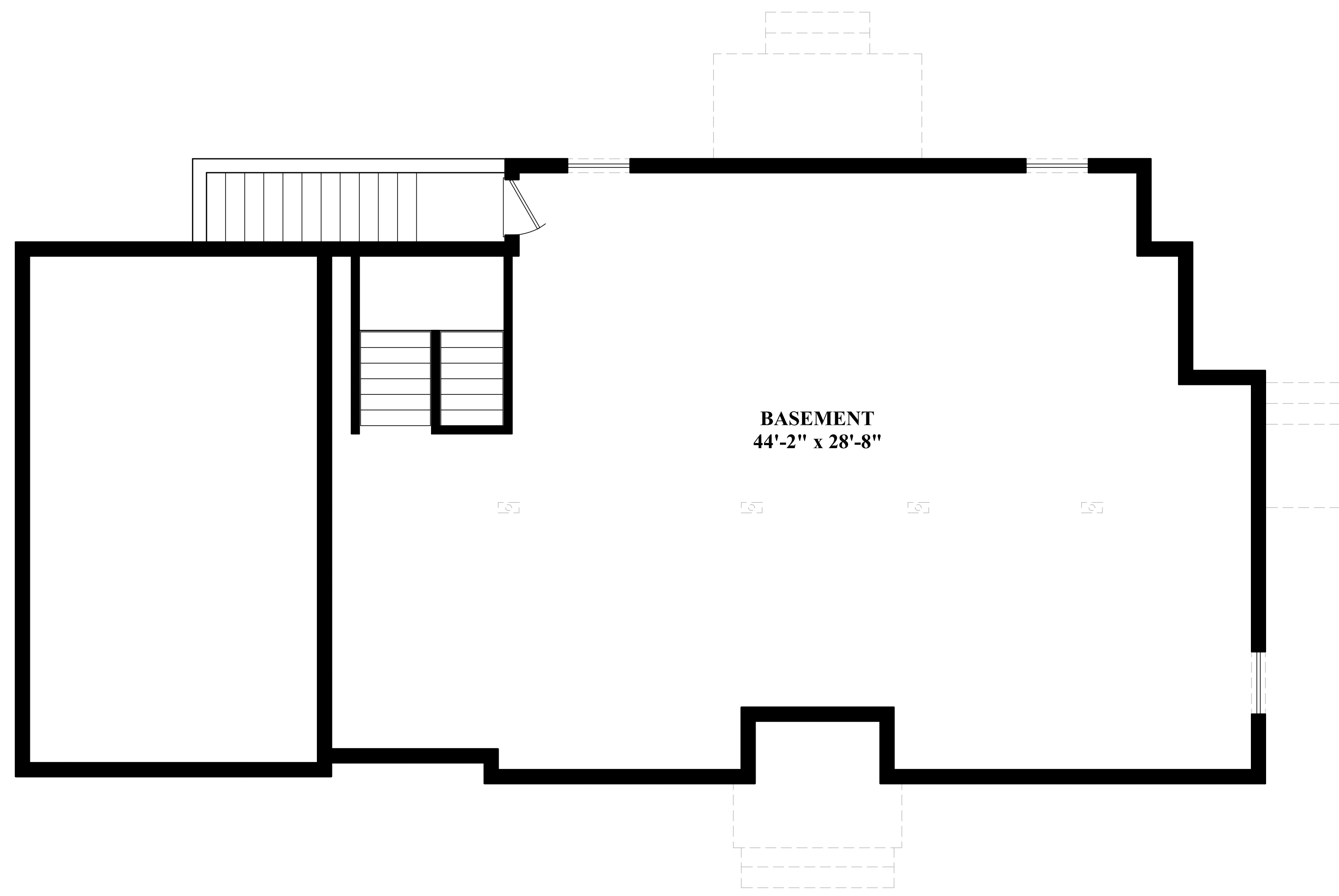
THE CATHERINE BASEMENT
